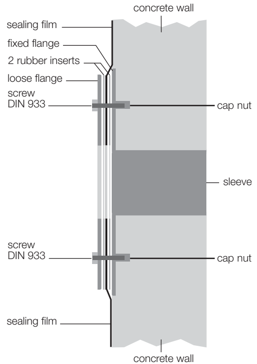
wall sleeve with fixed/loose flange according to DIN 18195 T 9 steel parts galvanized, alternatively stainless steel
