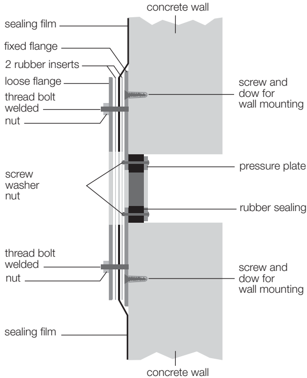
sealing with fixed/loose flange according to DIN 18195 T 9 steel parts galvanized, alternatively stainless steel
