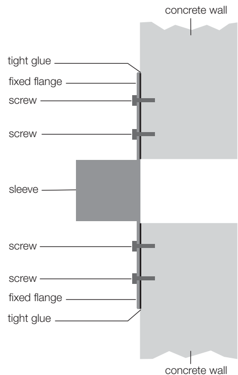
on wall-face sleeve in closed and split version, galvanized, alternatively stainless steel
