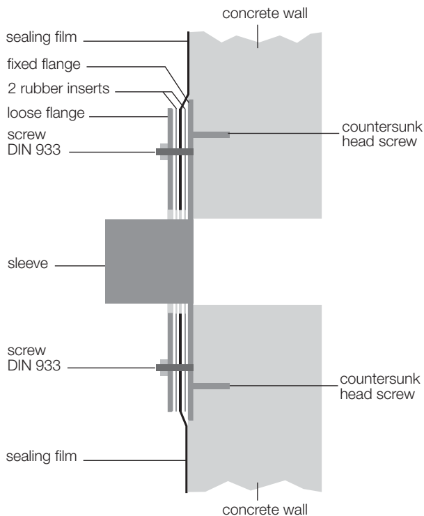
on wall-face sleeve with fix / loose flange according to DIN 18195 T 9, galvanized, alternatively stainless steel
